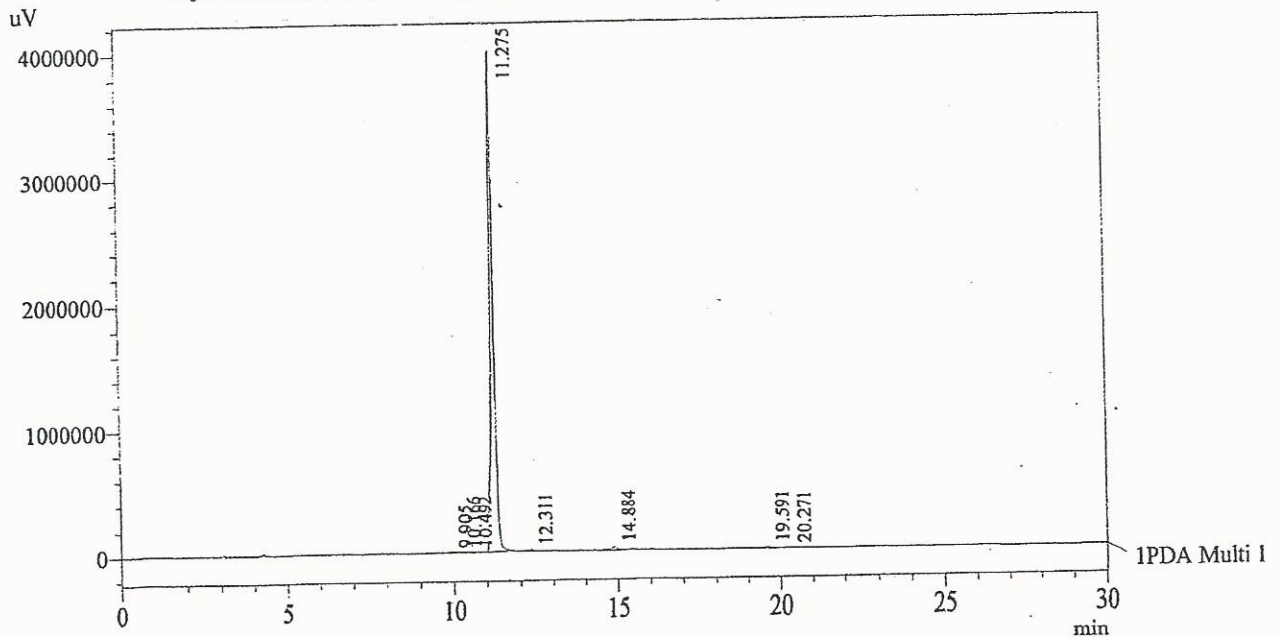
Chromatogram Myricetin (3,5,7,3',4',5'-Hexahydroxyflavone) D:\promonence\Data
